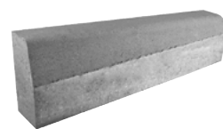
Via CL 1000 × 150 × 300 - 220 mm
